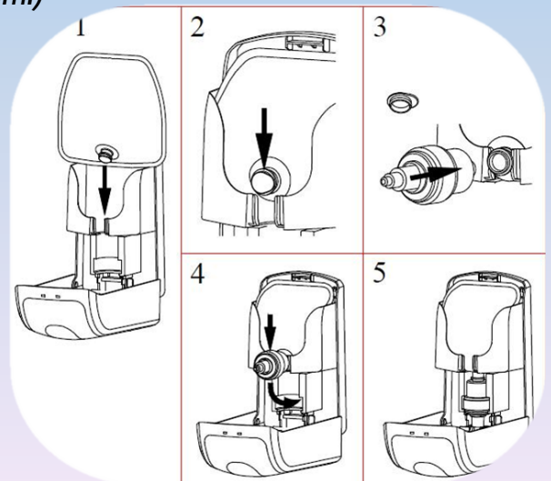
Bag installation instruction
